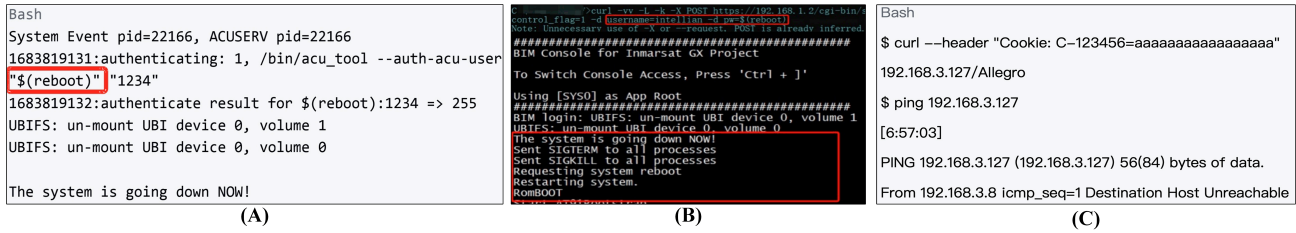
Figure 11: Examples of satellite modem attacks: (A) AC command injection; (B) Web command injection; (C) arbitrary write.
