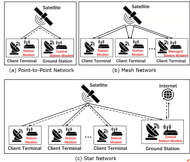
Figure 1: Three basic network architectures for satellite communication networks.
