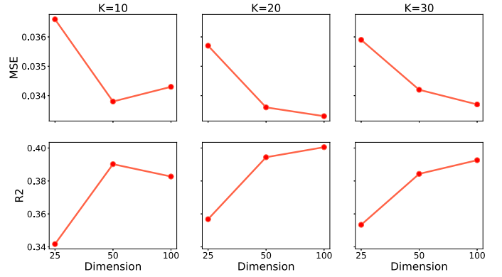
Fig. 5. Performance comparison on embedding sizes.
