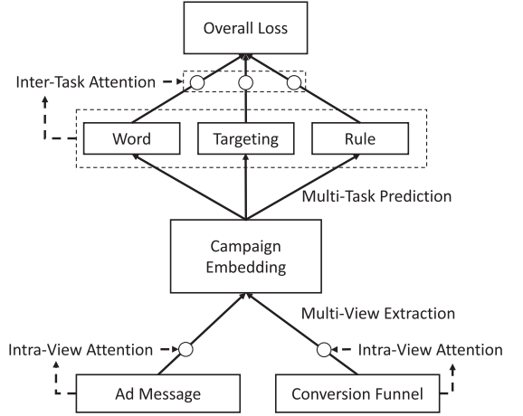
Fig. 2. Overview of campaign embedding framework.
